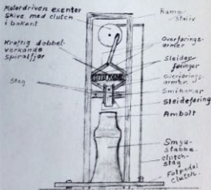
Prinsippskisse for motordriven smihamarlar 1938. Hans Klepp.
